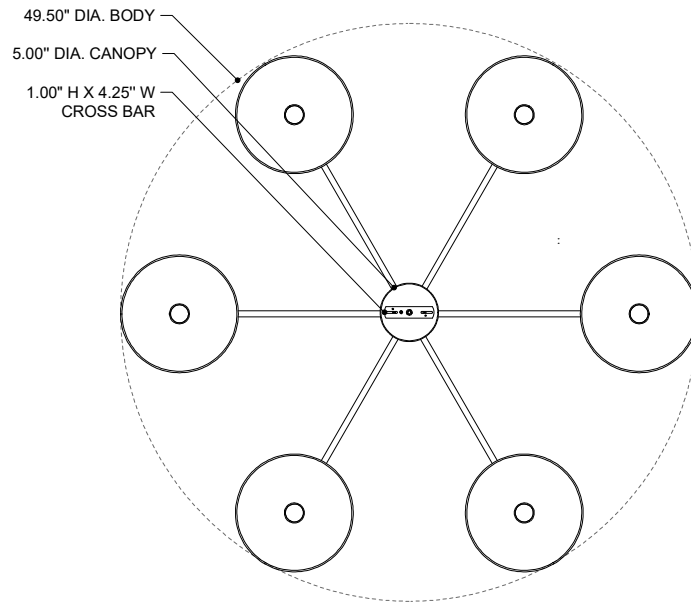
TOP VIEW
