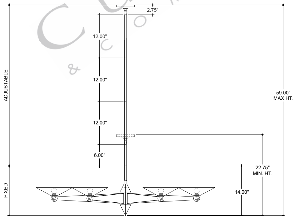
FRONT VIEW
