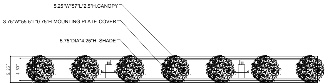
TOP VIEW
