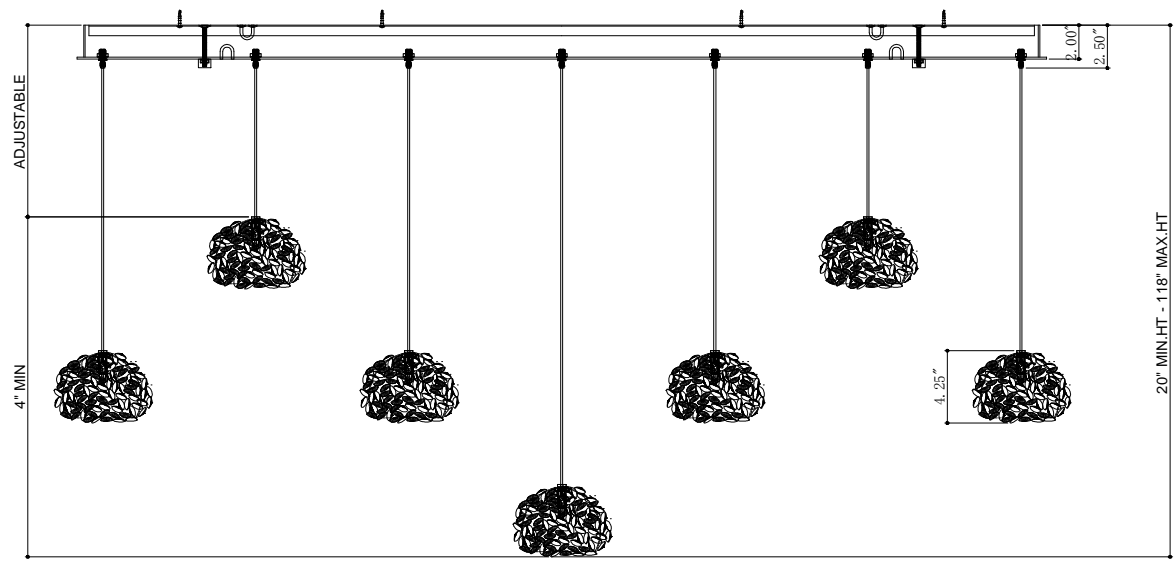
FRONT VIEW
