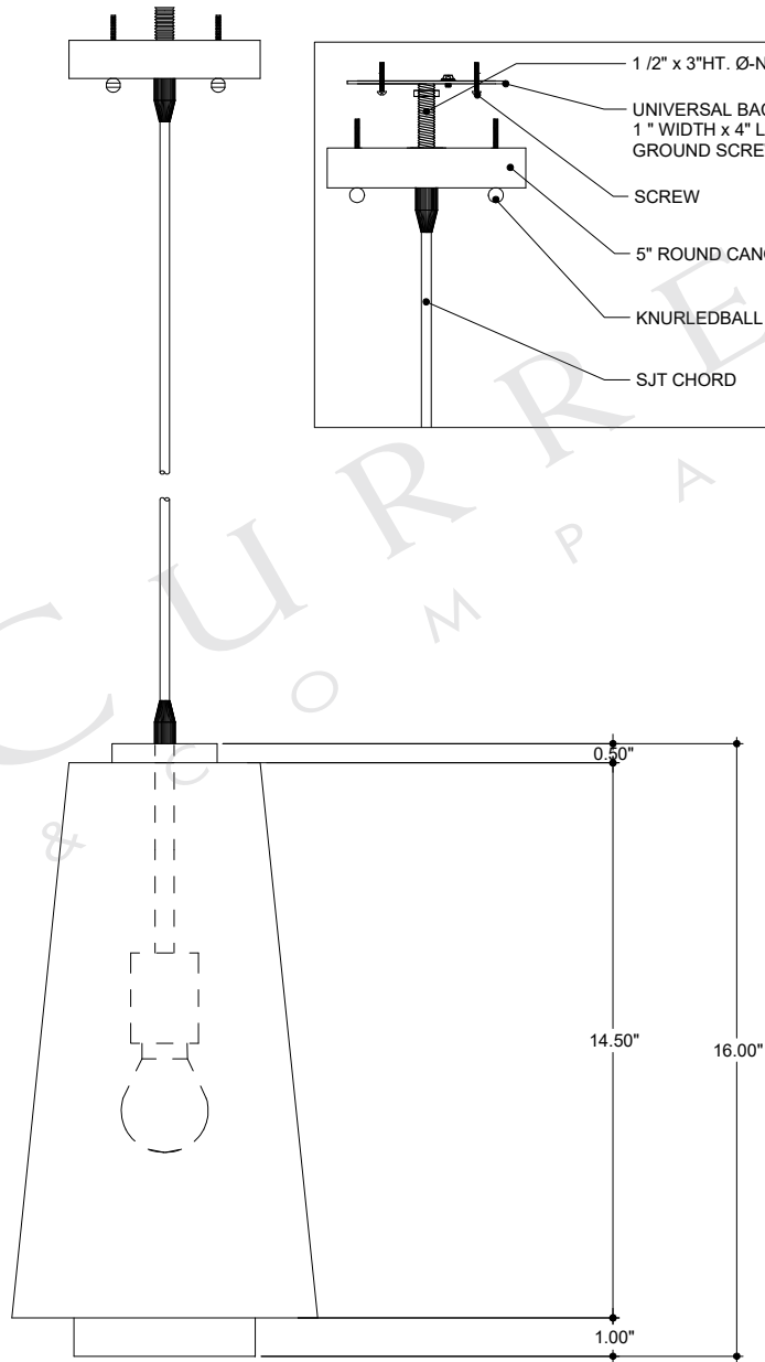
FRONT VIEW
