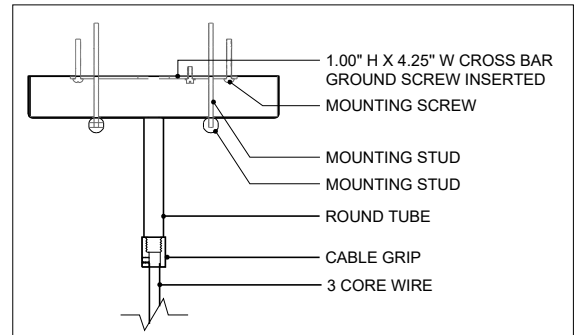
CANOPY DETAIL
