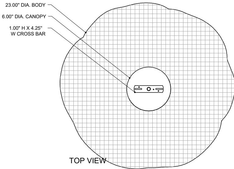
CANOPY DETAIL
