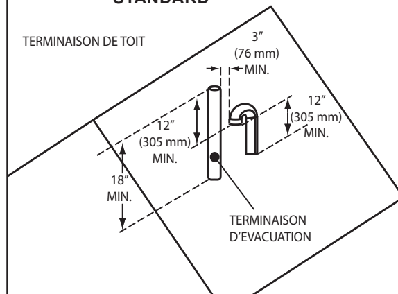
FIGURE 11 - CONFIGURATION D'ÉVACUATION VERTICALE STANDARD
