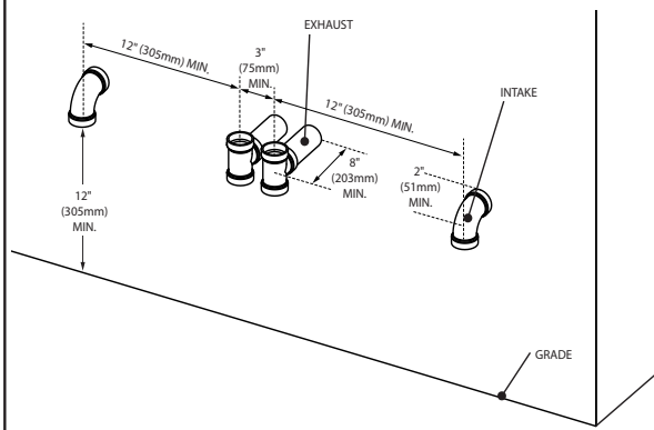
FIGURE 12 - MULTIPLE VENTING (STANDARD HORIZONTAL)
