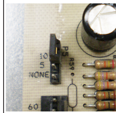
FIGURE 32 - JUMPER P5
