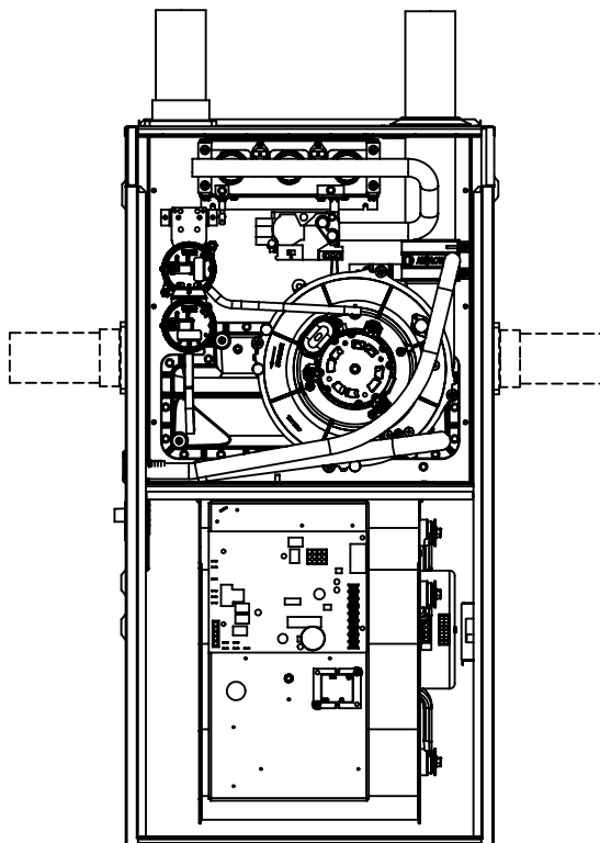
TOP VENT - LEFT DRAIN INSTALLATION (INTERNAL)
