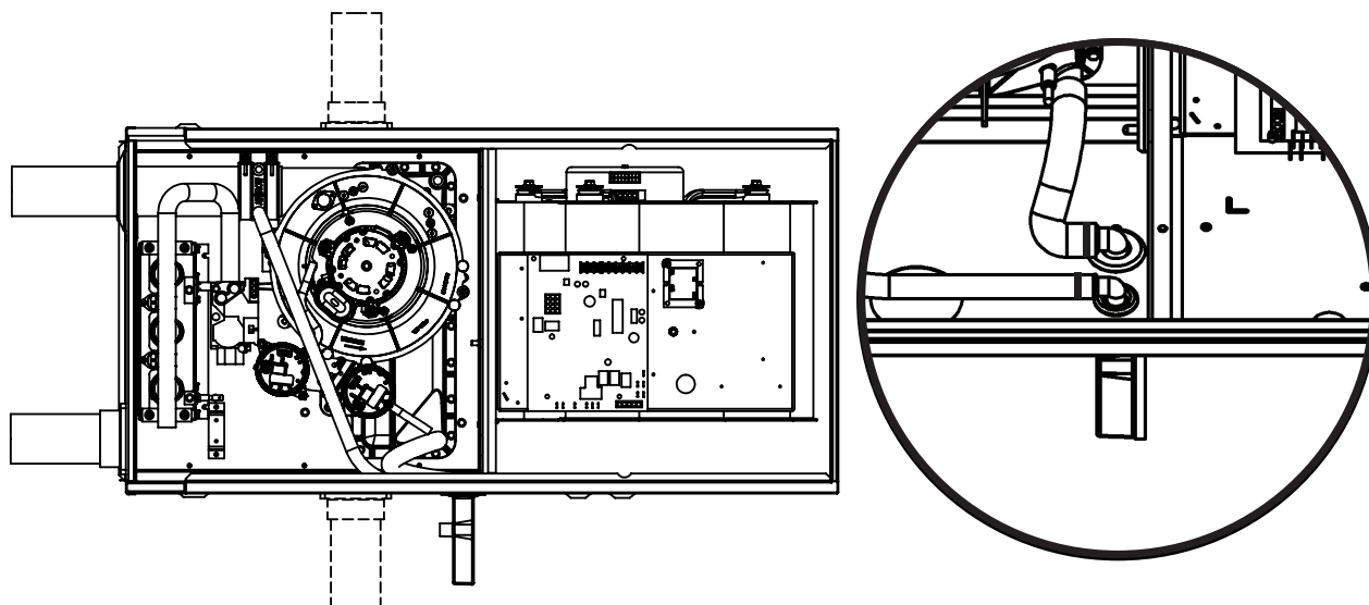
FIGURE 17 - HORIZONTAL LEFT VENT AND DRAINING OPTION
