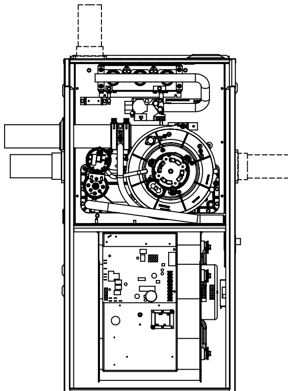
LEFT VENT - RIGHT DRAIN INSTALLATION (INTERNAL)
