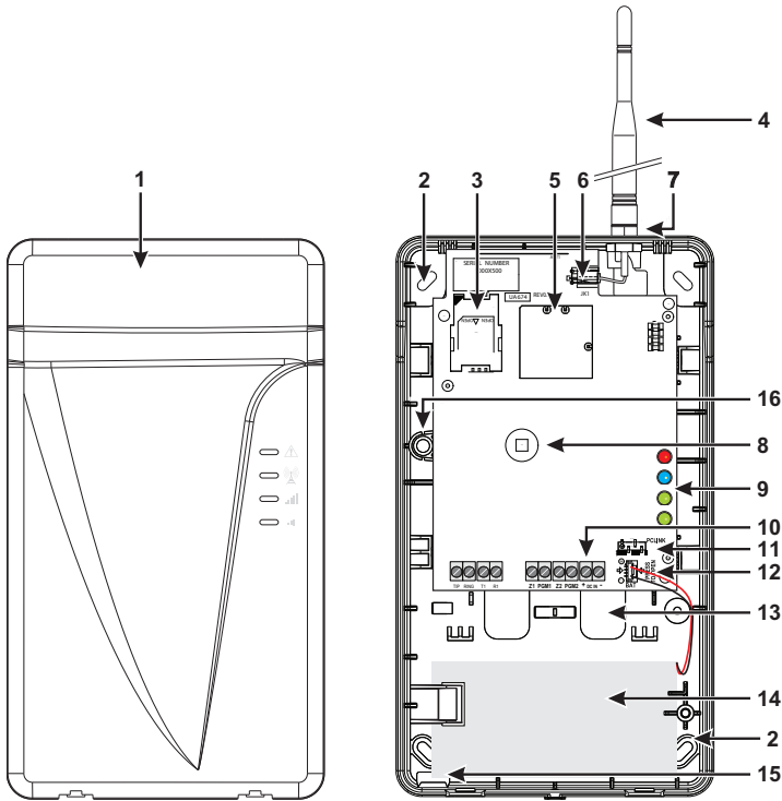
Figure 1 - Parts
