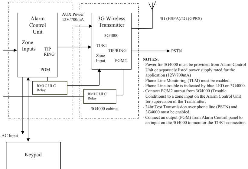
Figure 5 - Alarm Control Unit and 3G Transmitter
