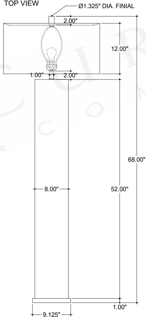
FRONT VIEW
