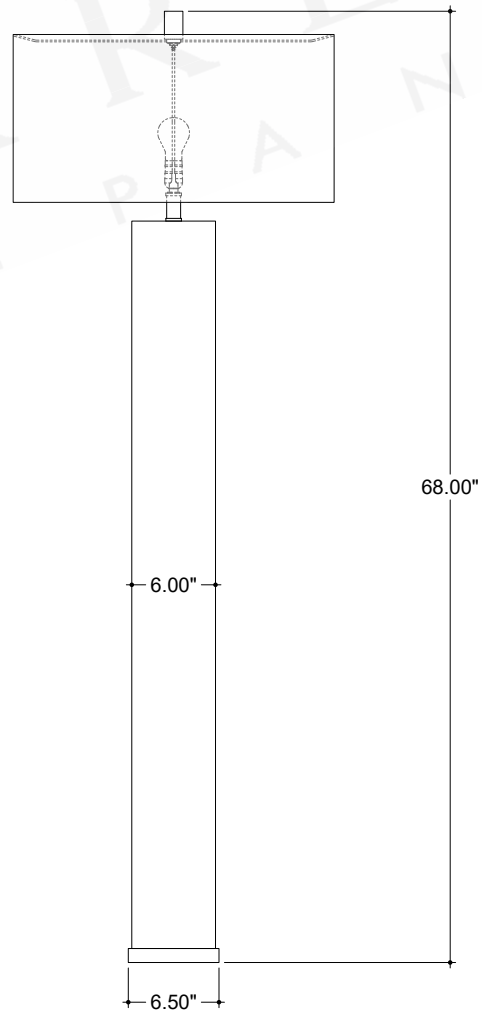
SIDE VIEW
