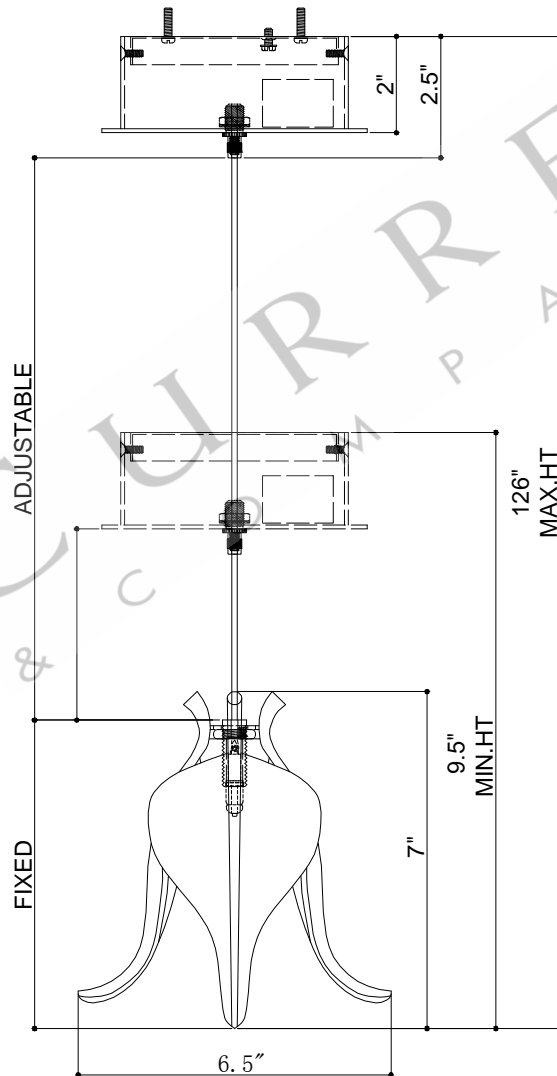
FRONT VIEW
