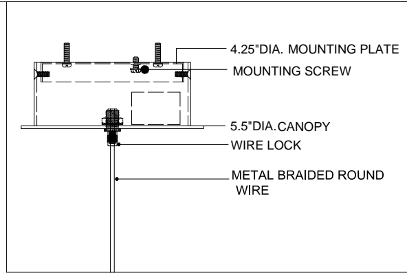
CANOPY DETAIL
