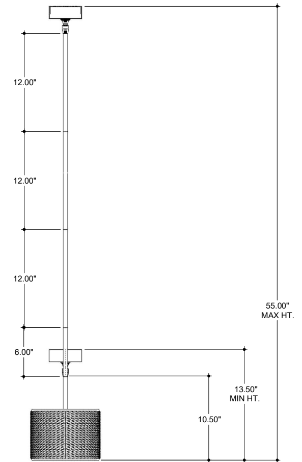
SIDE VIEW
