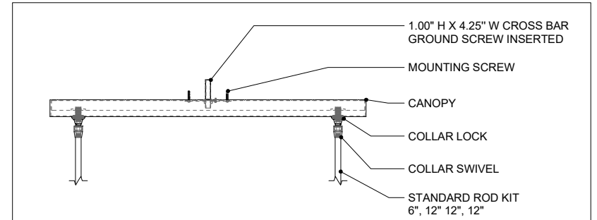
CANOPY DETAIL
