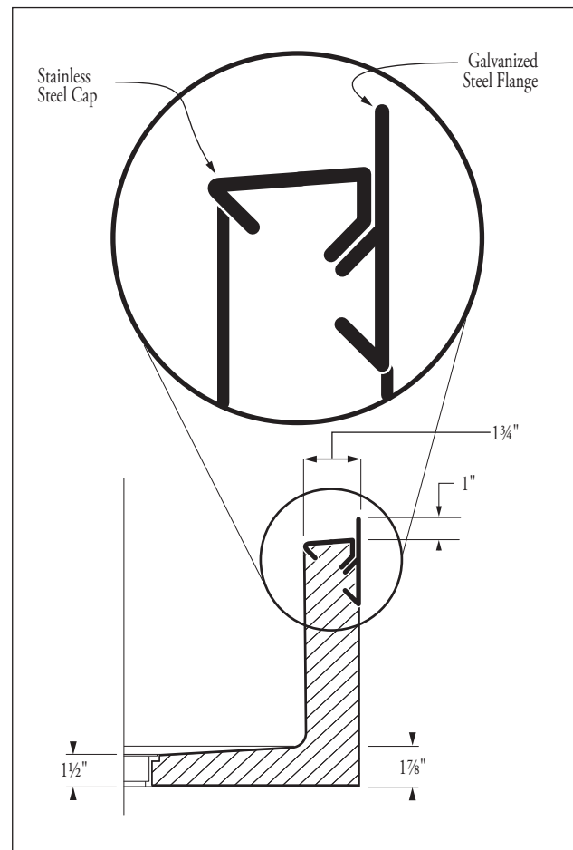
Construction Detail showing optional flange and cap.
