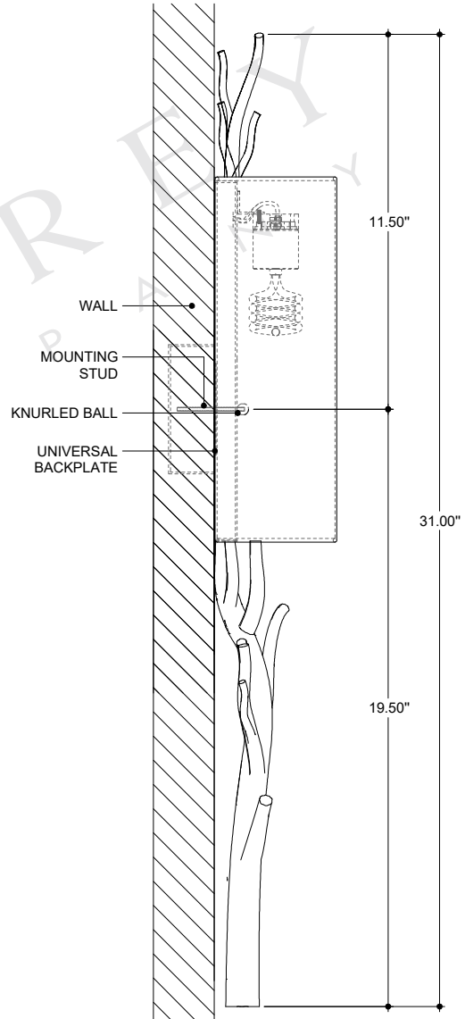
SIDE VIEW
