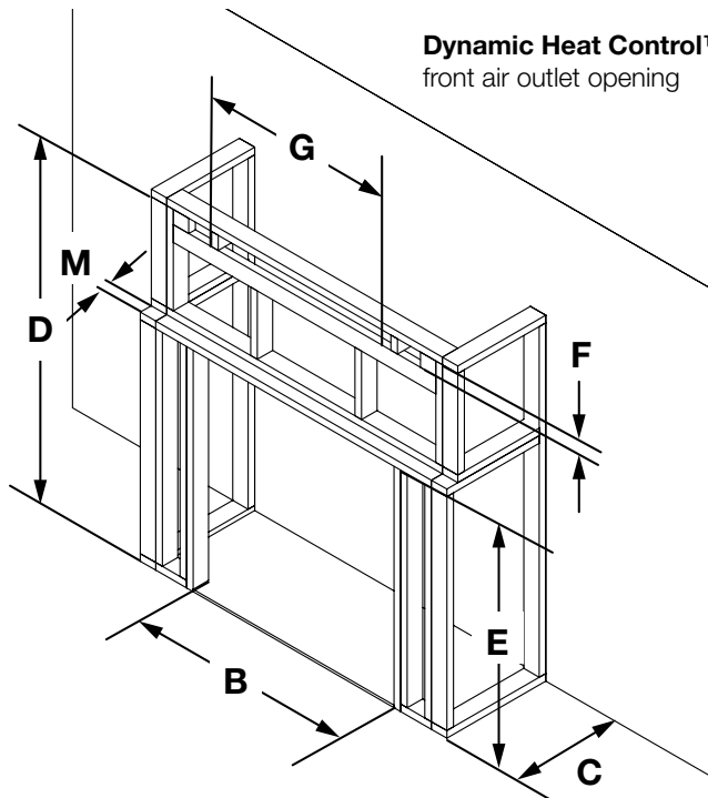
Installation Option 2 illustrated
