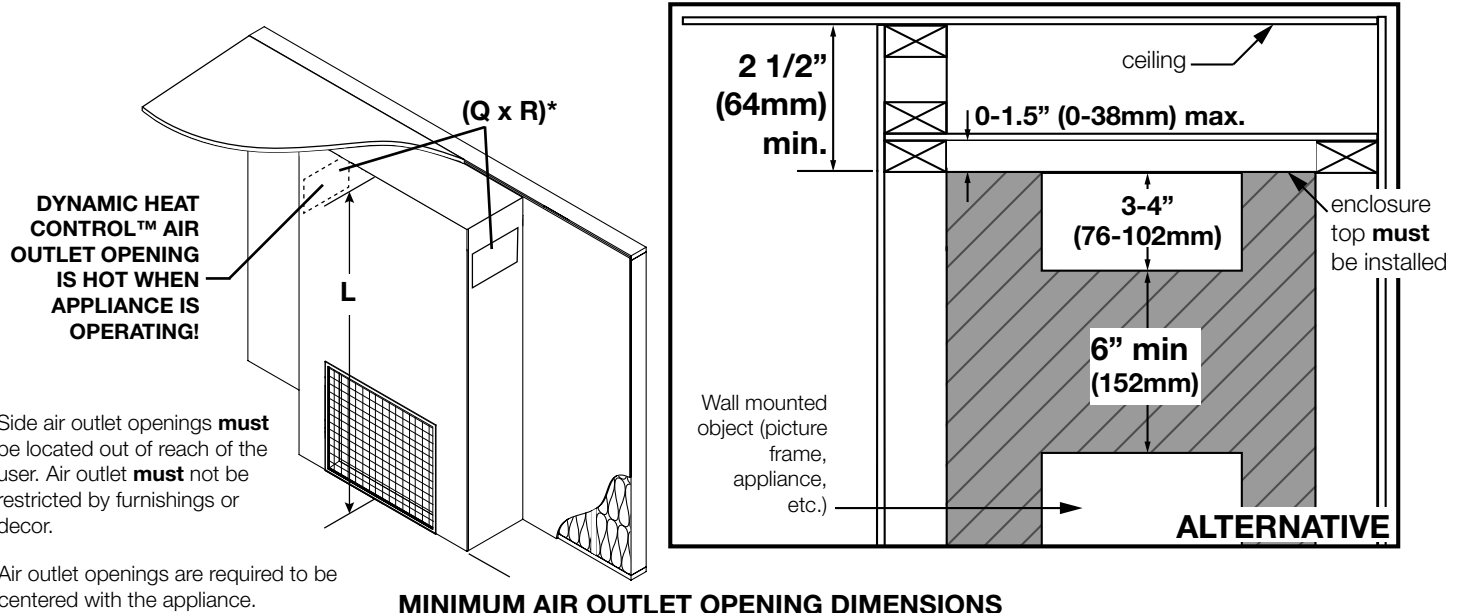
MINIMUM AIR OUTLET OPENING DIMENSIONS
