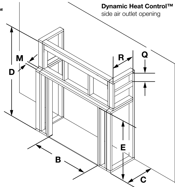
Installation Option 5 illustrated
