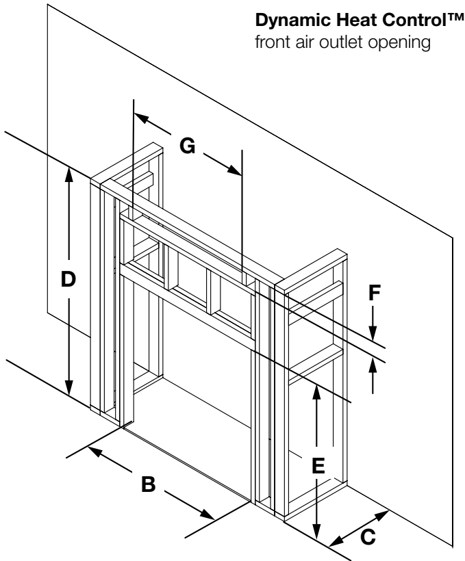
Installation Option 2 illustrated
