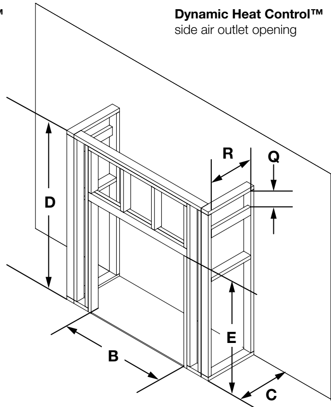
Installation Option 5 illustrated
