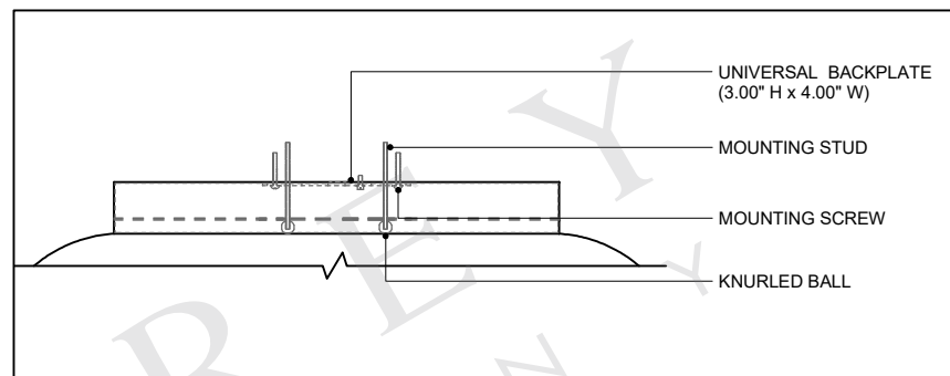
CANOPY DETAIL
