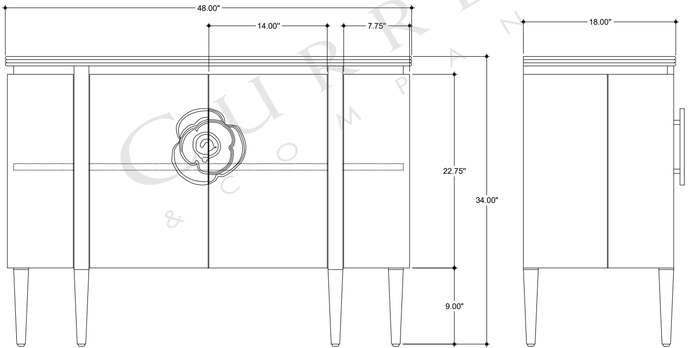
FRONT VIEW
