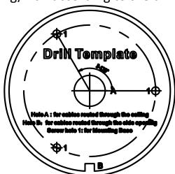
Figure 2-1 Drill Template
