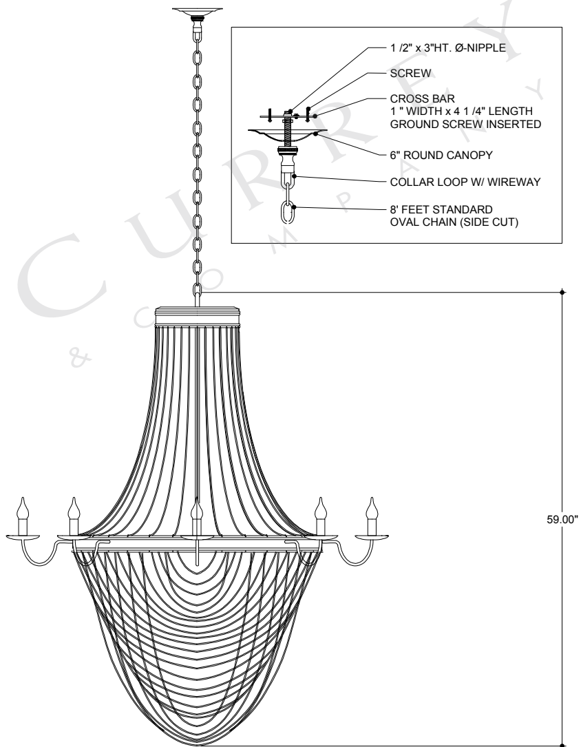
FRONT VIEW
