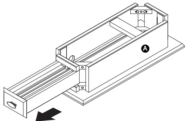
Top Assembly
