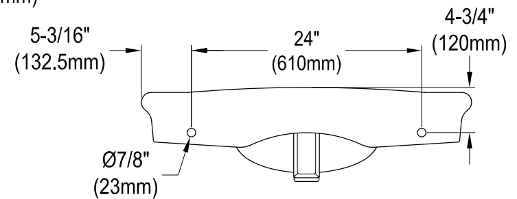
Sink Back View
