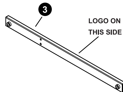
LOWER BOARD ARM ASSEMBLY, LH 1A-7954-10 QTY. 1
