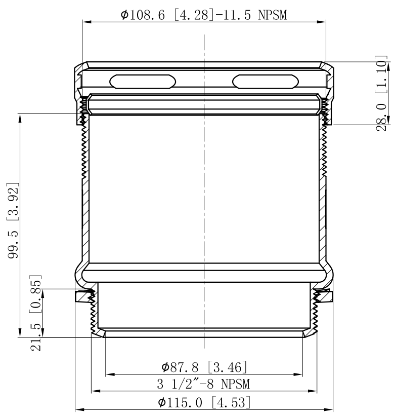
CUTAWAY VIEW A-A
