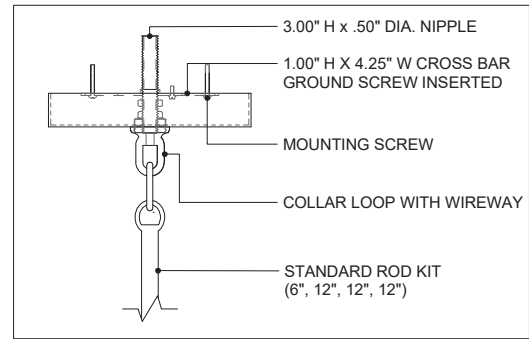
CANOPY DETAIL
