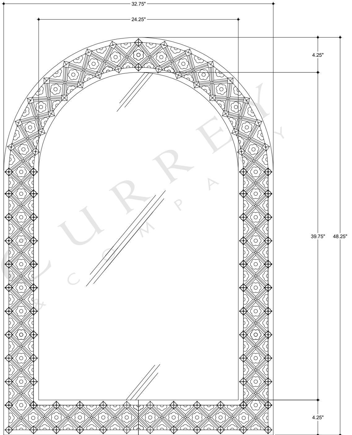
FRONT VIEW
