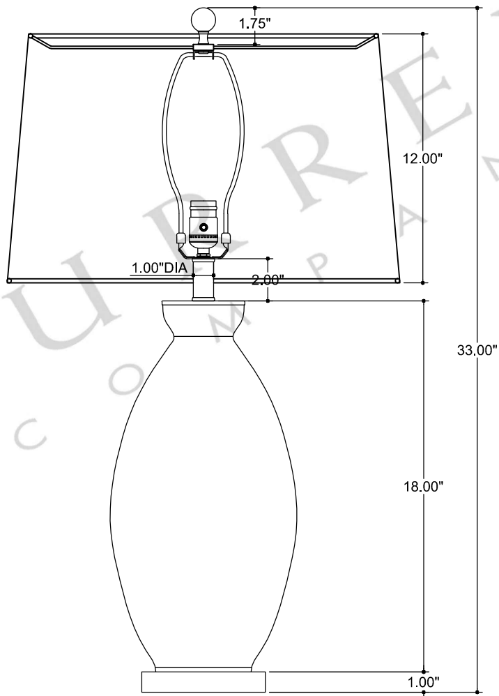
FRONT VIEW
