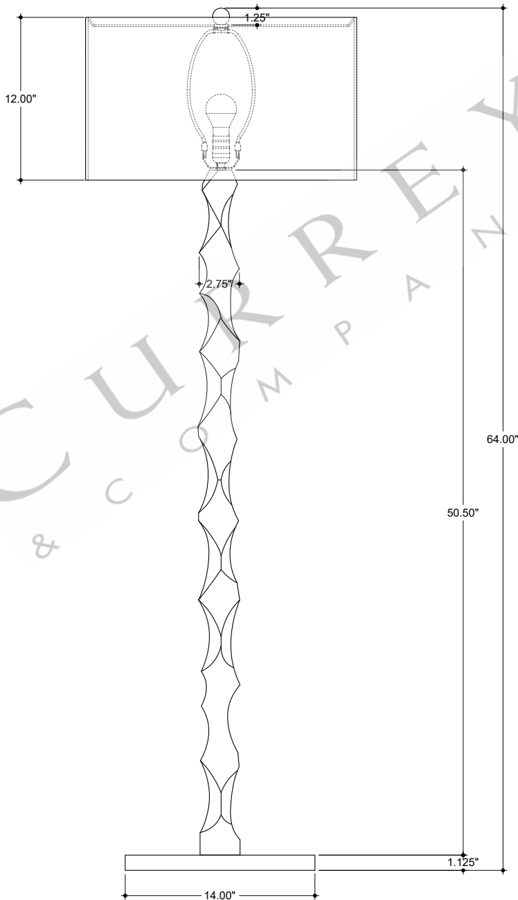
FRONT VIEW
