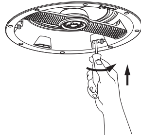
Repeat for the other two Swiftlock™ mounting dogs
