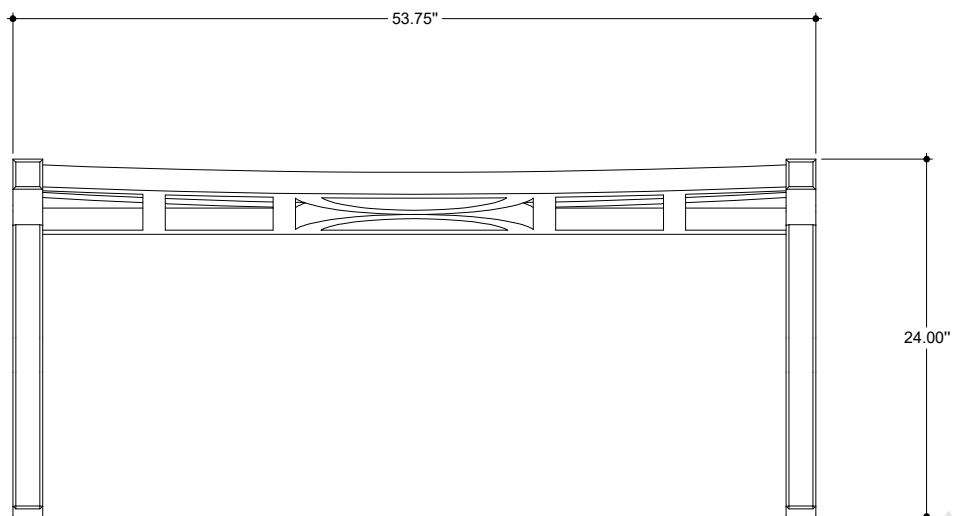
TOP VIEW
