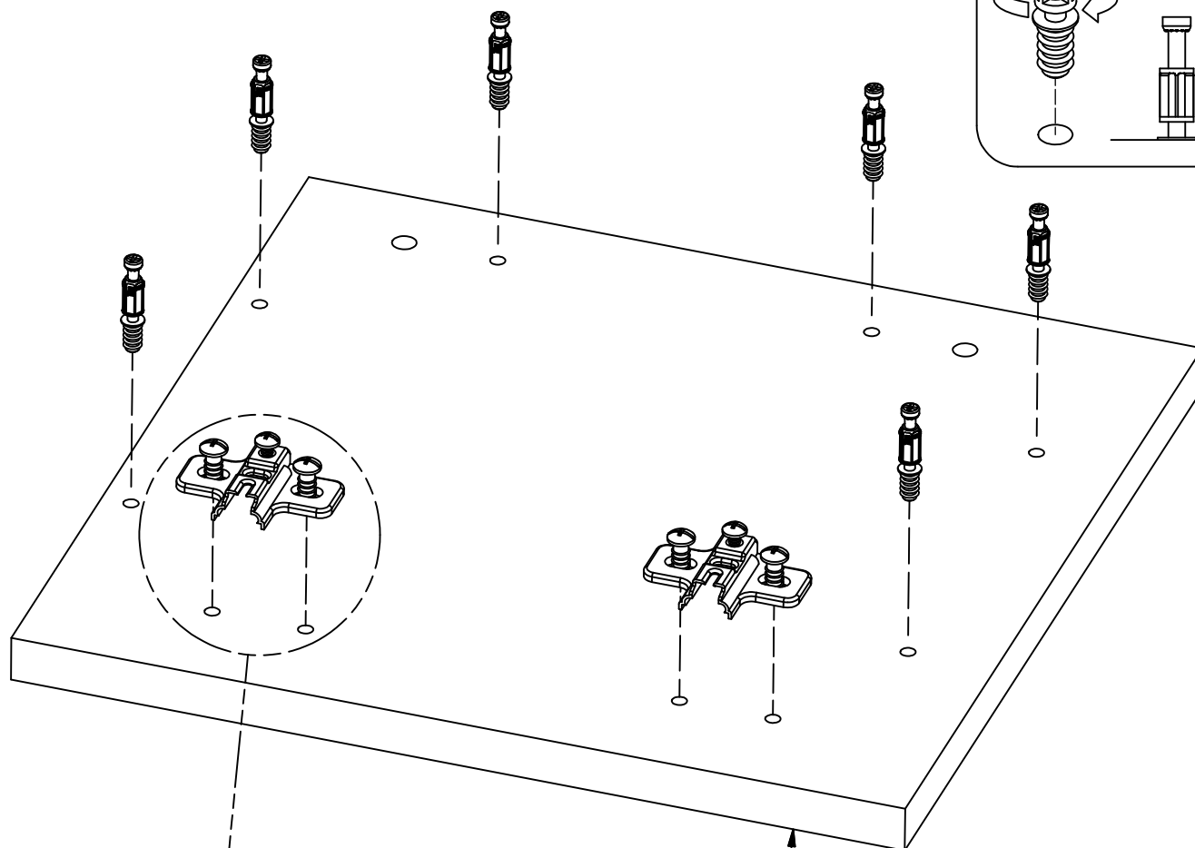
Mounting Plate
