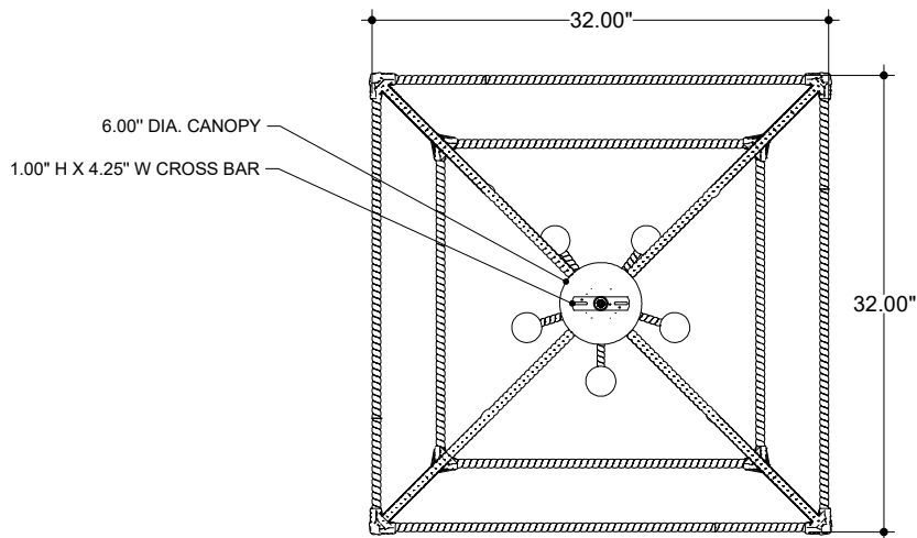
CANOPY DETAIL
