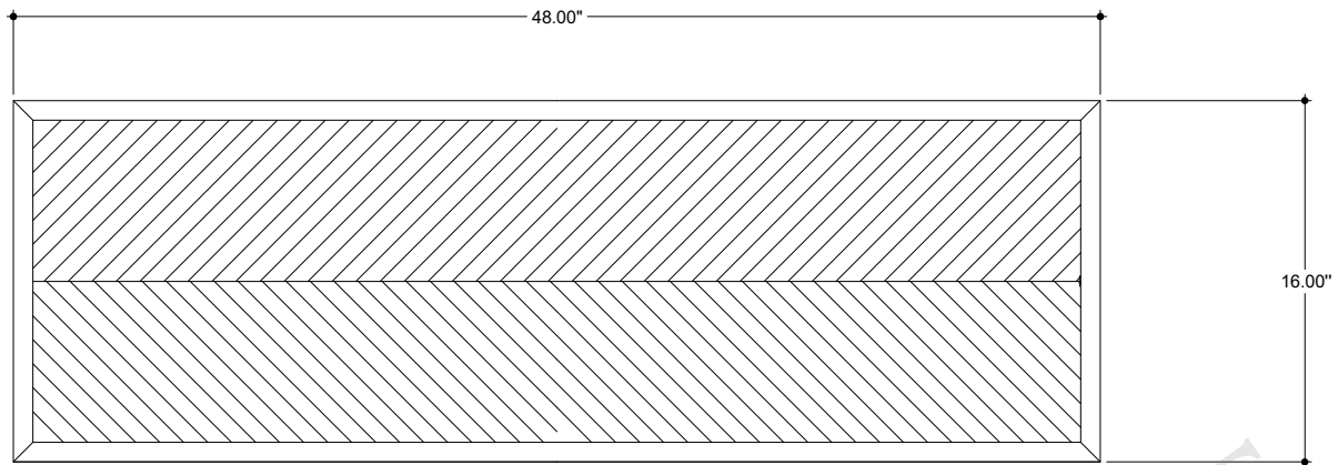
TOP VIEW
