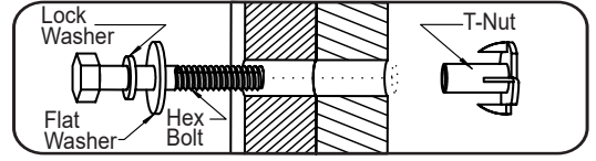
Hex Bolt Assembly
