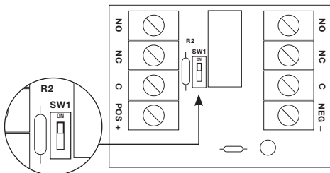
SW1 DIP Switch
