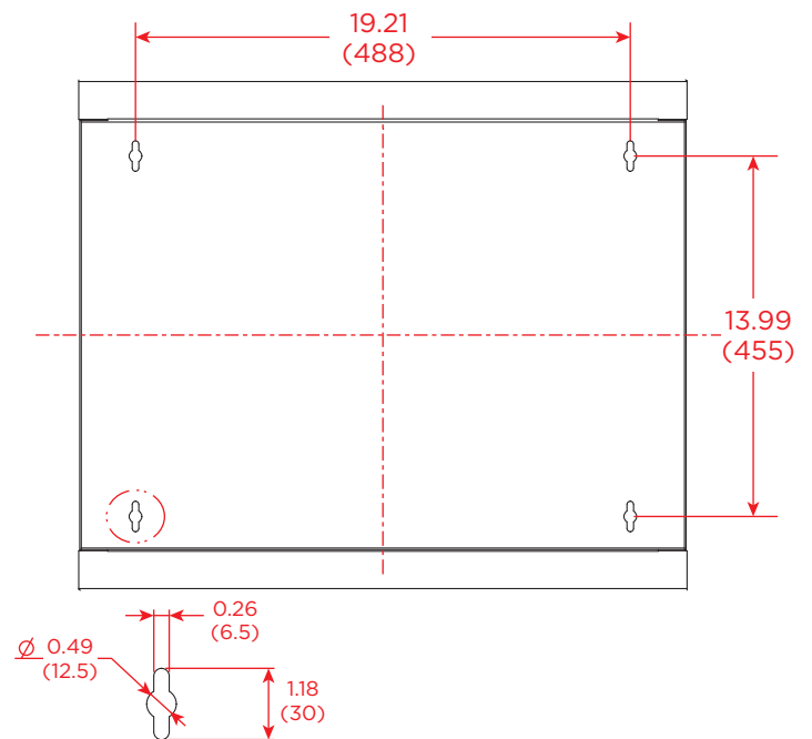
REAR VIEW
