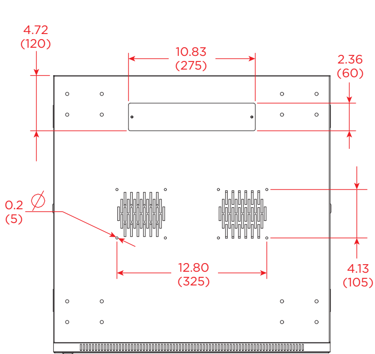
TOP/BOTTOM VIEW
