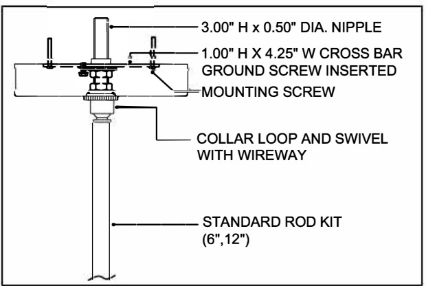
CANOPY DETAIL
