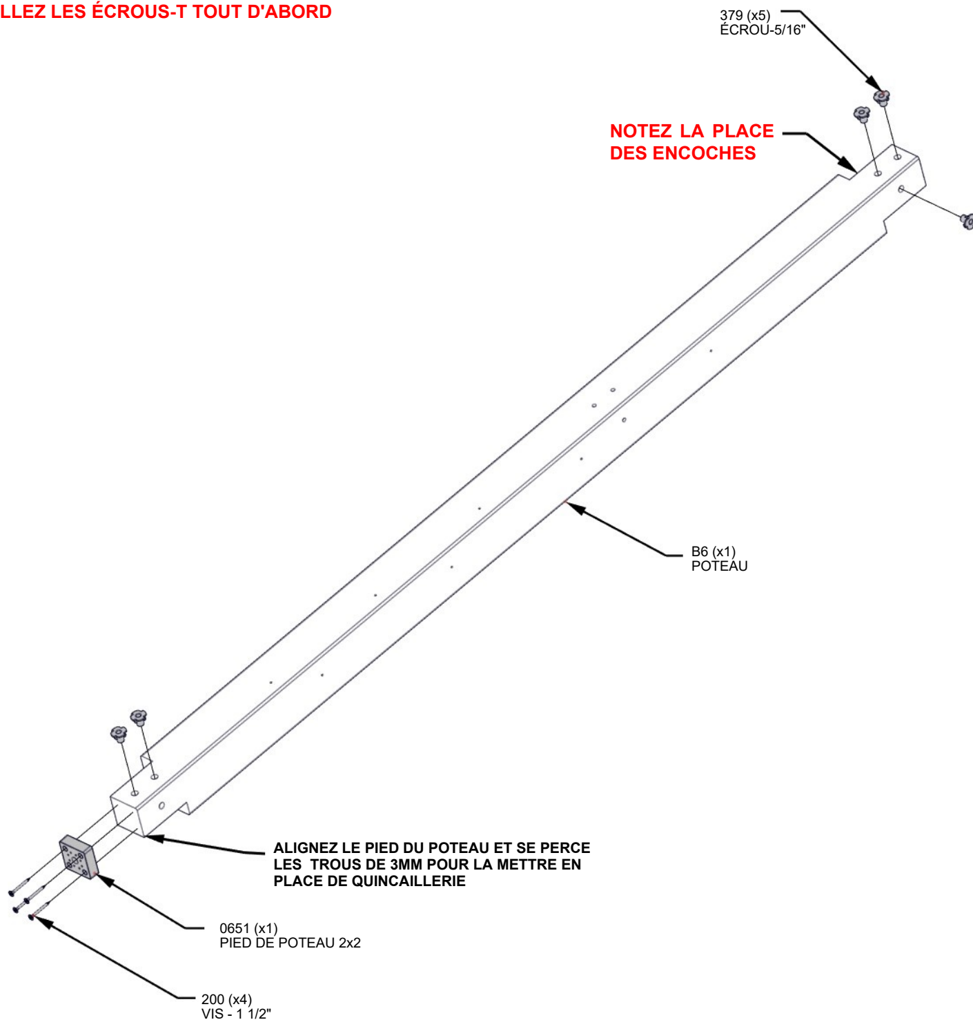
A6P00651 PIED DE POTEAU 2x2 (x1)
