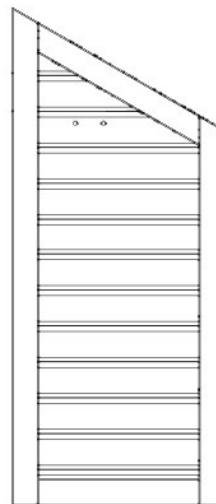
WP5 PANNEAU MURAL-W2A04048 (x1) 1 1/16"X19 1/16"X55 5/8" (27x484x1412)
