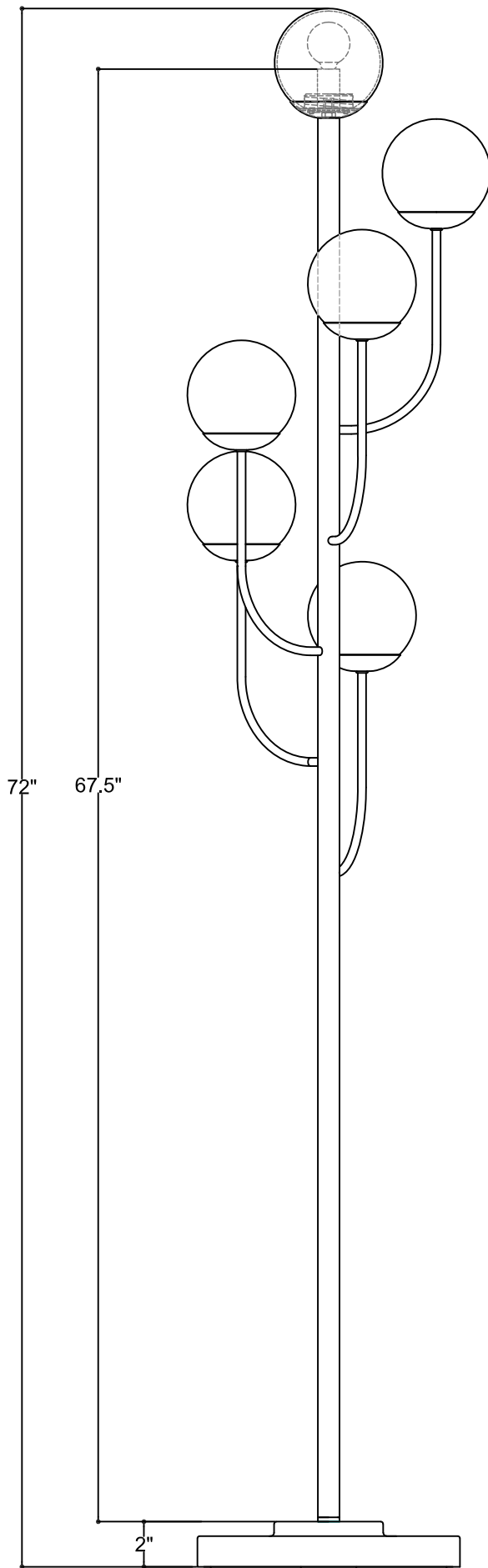
FRONT VIEW
