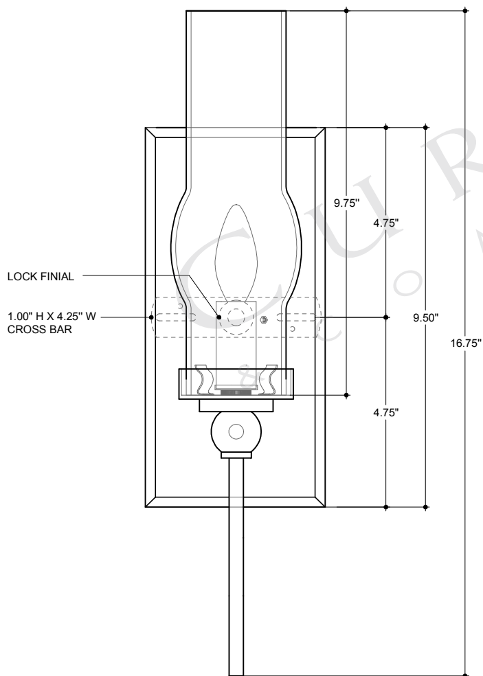
FRONT VIEW
