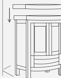
② Install Counter Top.
