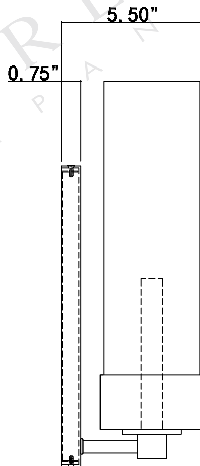
SIDE VIEW
