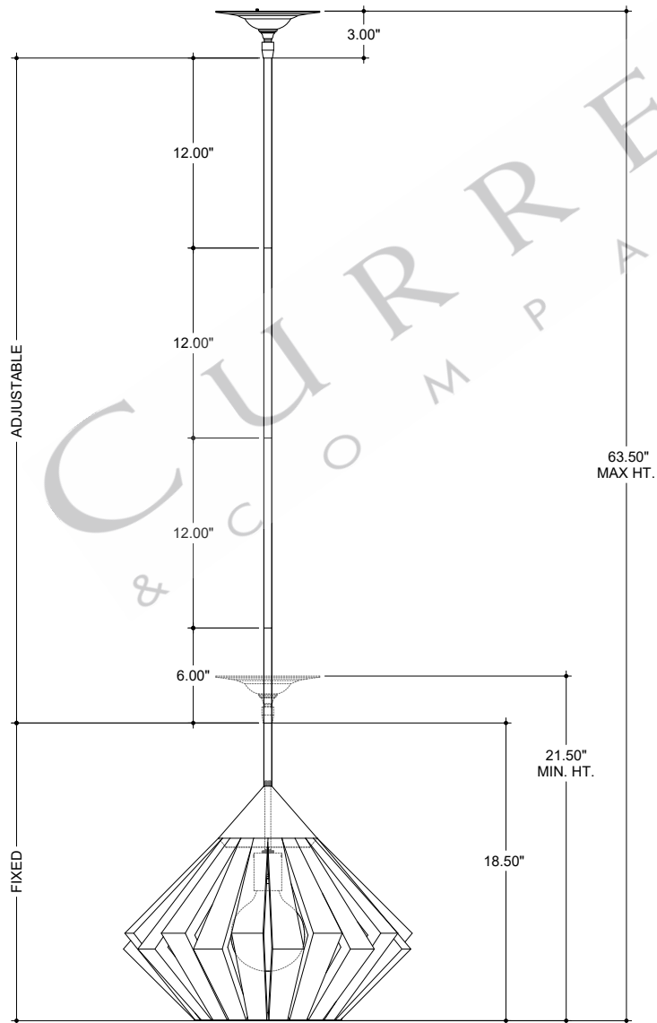
FRONT VIEW
