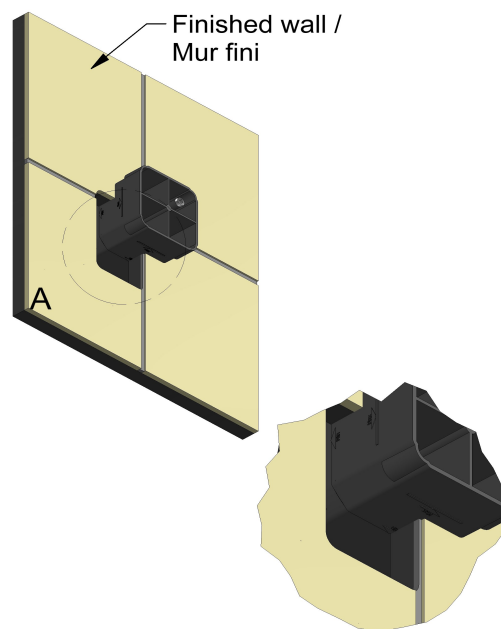
DETAIL A
