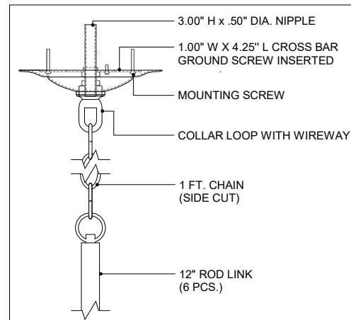
CANOPY DETAIL
