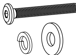
ALLEN KEY BOLT: M8 X 50mm - QTY 8 LOCK WASHER: \varnothing 12 / \varnothing 8 \times 1.5\text{mm} - QTY 8 WASHER: \varnothing 19 / \varnothing 8 \times 1\text{mm} - QTY 8 QTY 8 SETS
