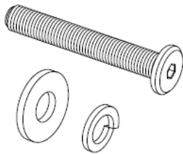
ALLEN KEY BOLT M8 x 60 mm LOCK WASHER Ø 12 / Ø 8 x 1.5 mm WASHER Ø 19 / Ø 8 x 1 mm QTY 8 SETS
