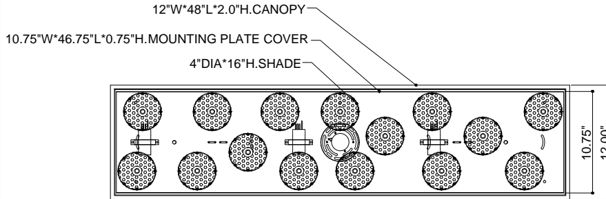
TOP VIEW
