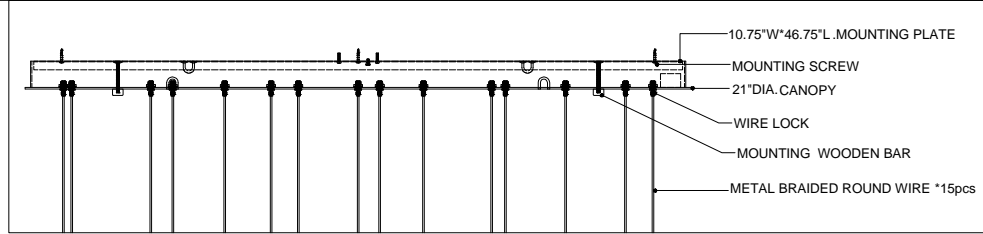
CANOPY DETAIL
