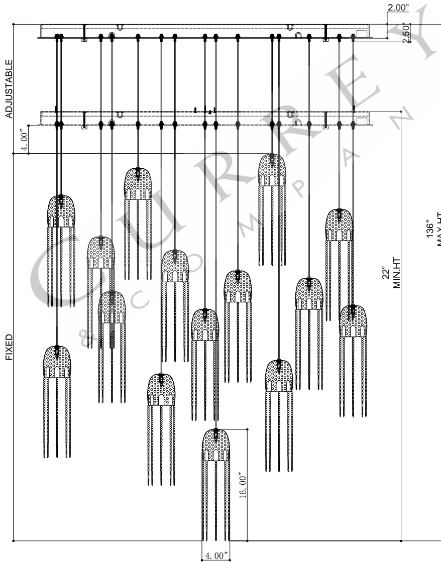
FRONT VIEW
