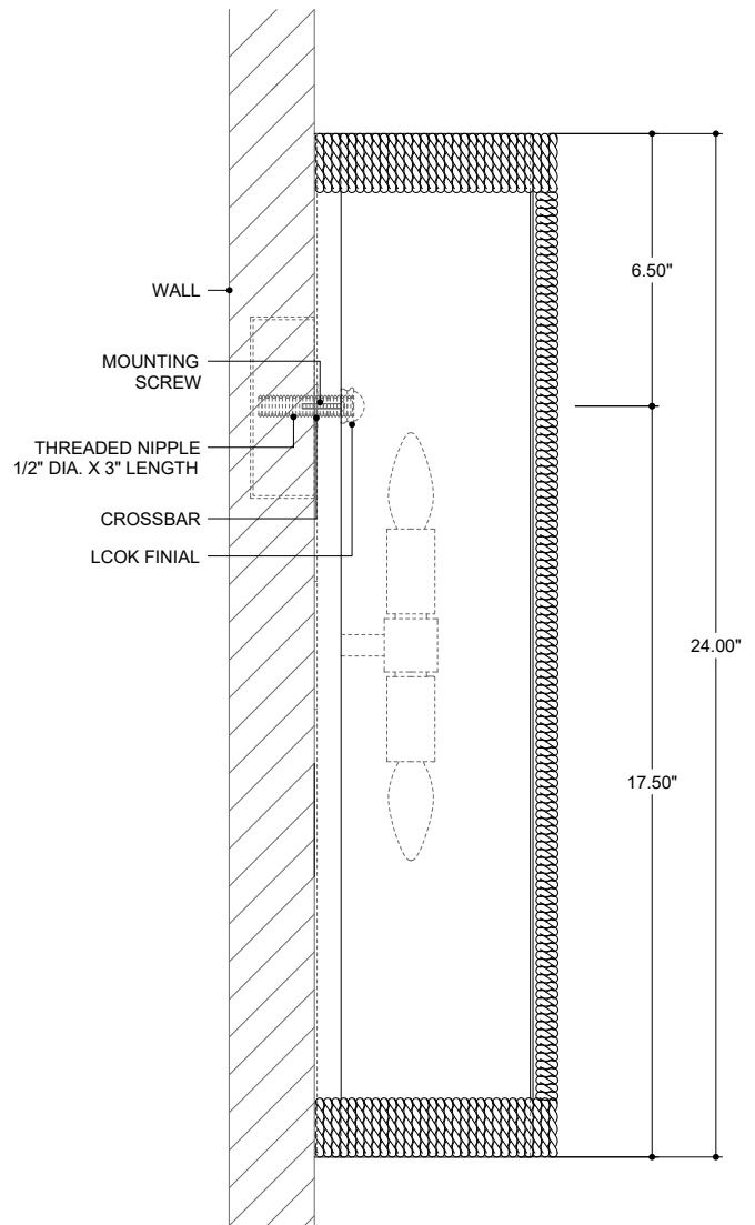
SIDE VIEW
