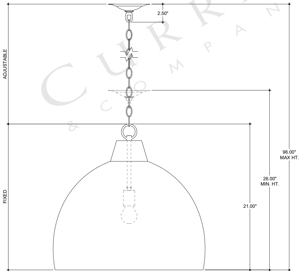
FRONT VIEW
