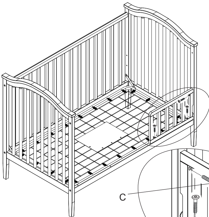
C. M6x45 mm Φ17 Head Bolt x1 Part #5587
