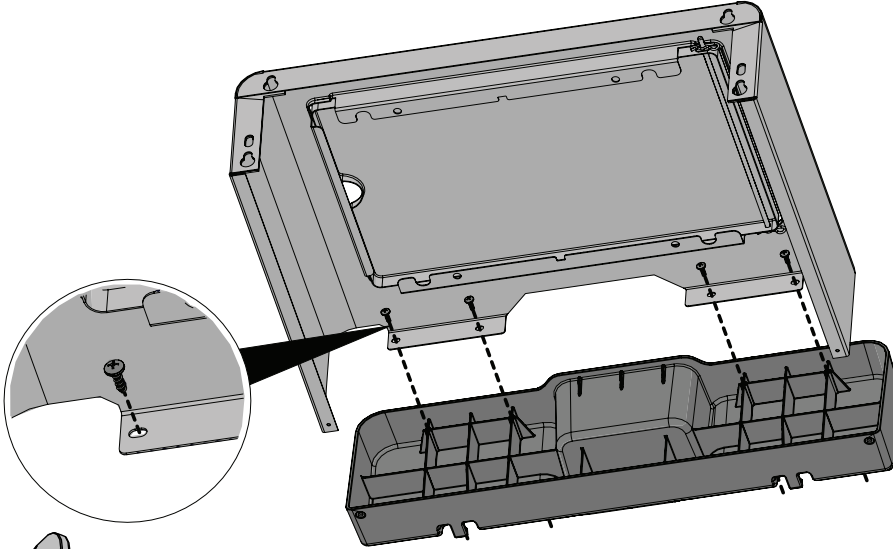
N570-0076 (#8 X 1/2")
