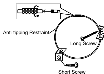
Anti-Tipping Device 1 set
