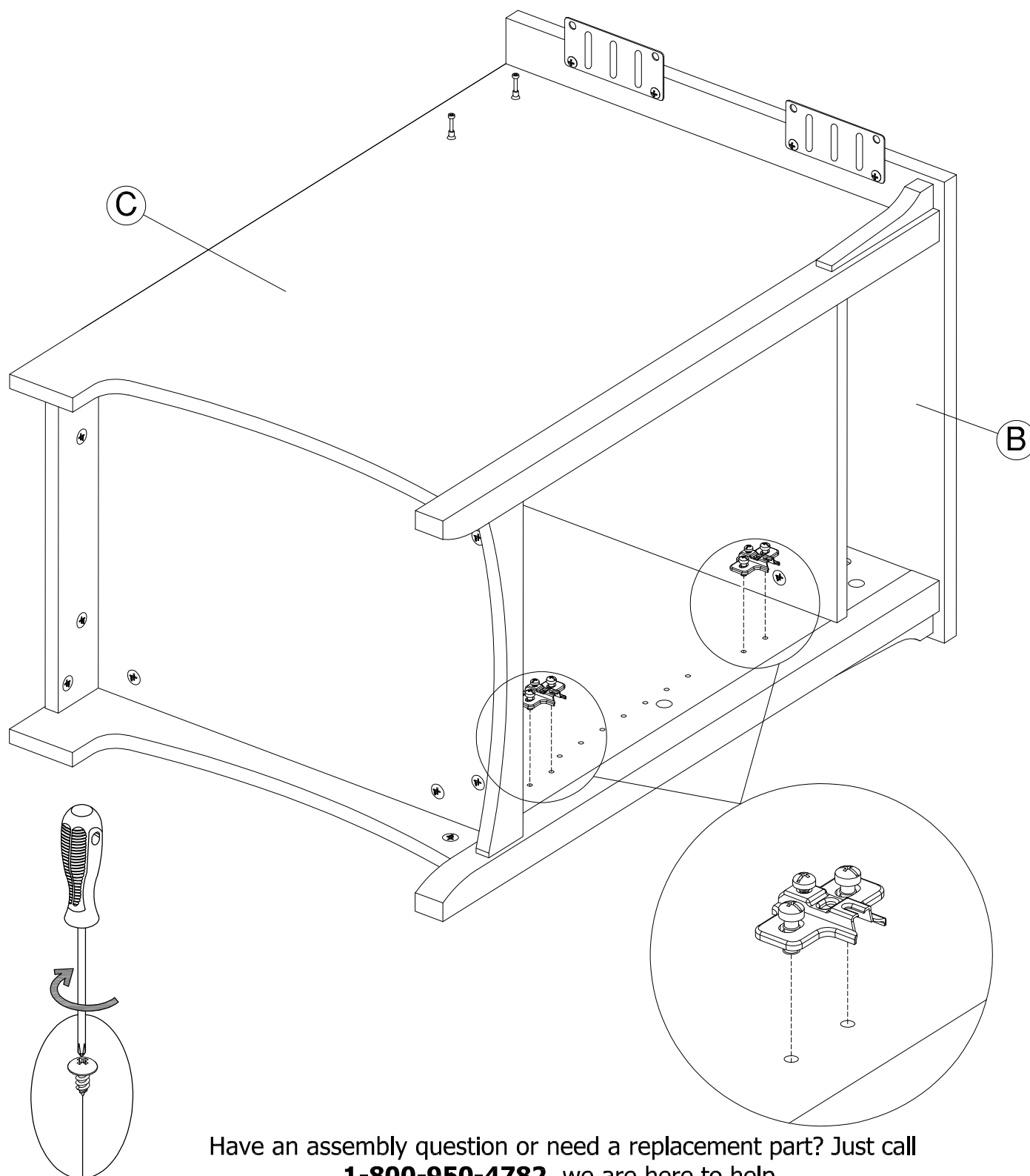
Mounting Plate
